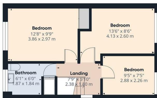
Floor 1
